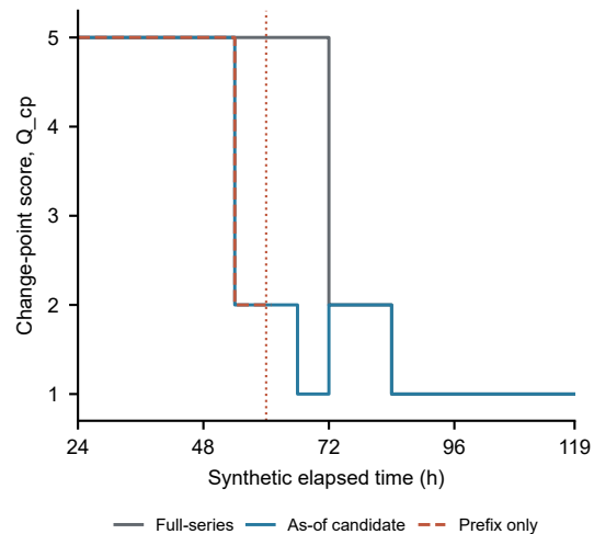
(b) D4: future candidates alter past scores
