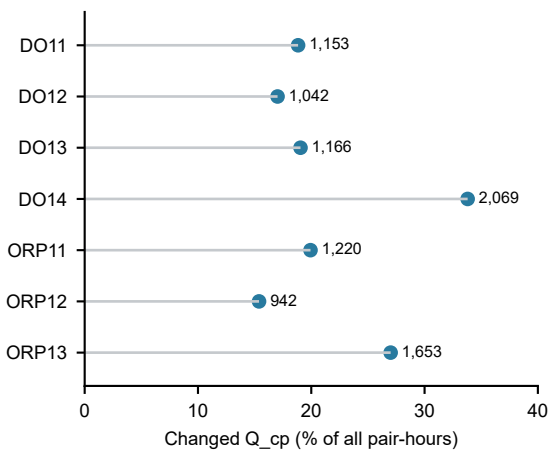
(c) Old-period change-point score differences
