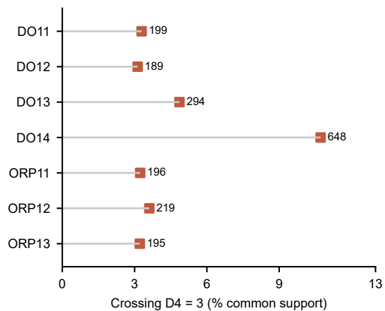
(d) Low-tail flips with other evidence fixed
